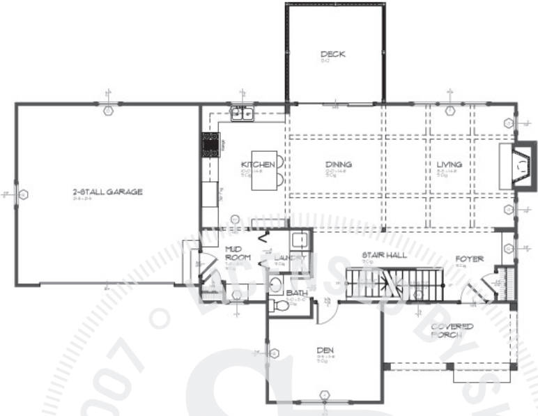
MAIN FLOOR 1080 SQ FT © Copyright 2006. Licensed by Sketchpad Inc.
