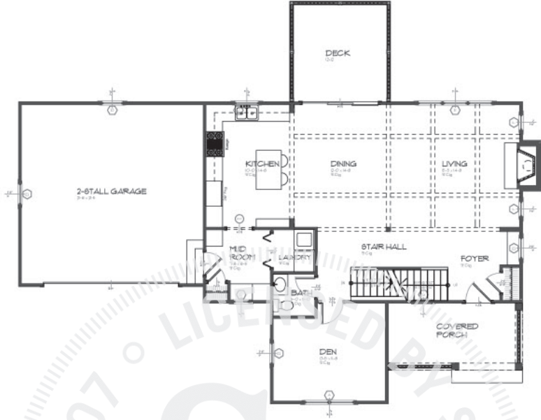
MAIN FLOOR
